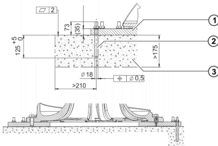
Fig. 6-3: Cross-section of foundation 175 mm
