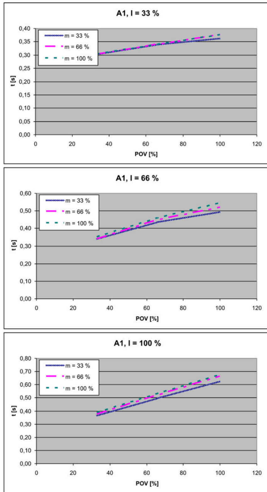
Fig. 4-12: Stopping times for STOP 1, axis 1
