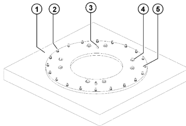
Fig. 8-1: Mounting base 175 mm
