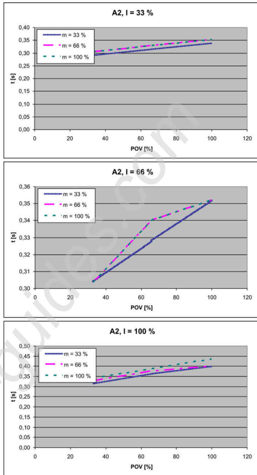
Fig. 4-14: Stopping times for STOP 1, axis 2
