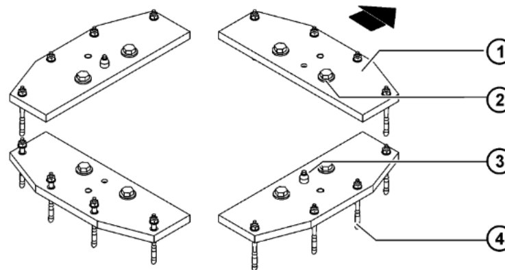
Fig. 8-4: Mounting base 200 mm
