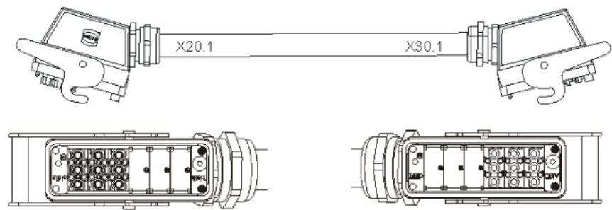
Fig. 8-10: Connecting cable, motor cable, X20.1 - X30.1
