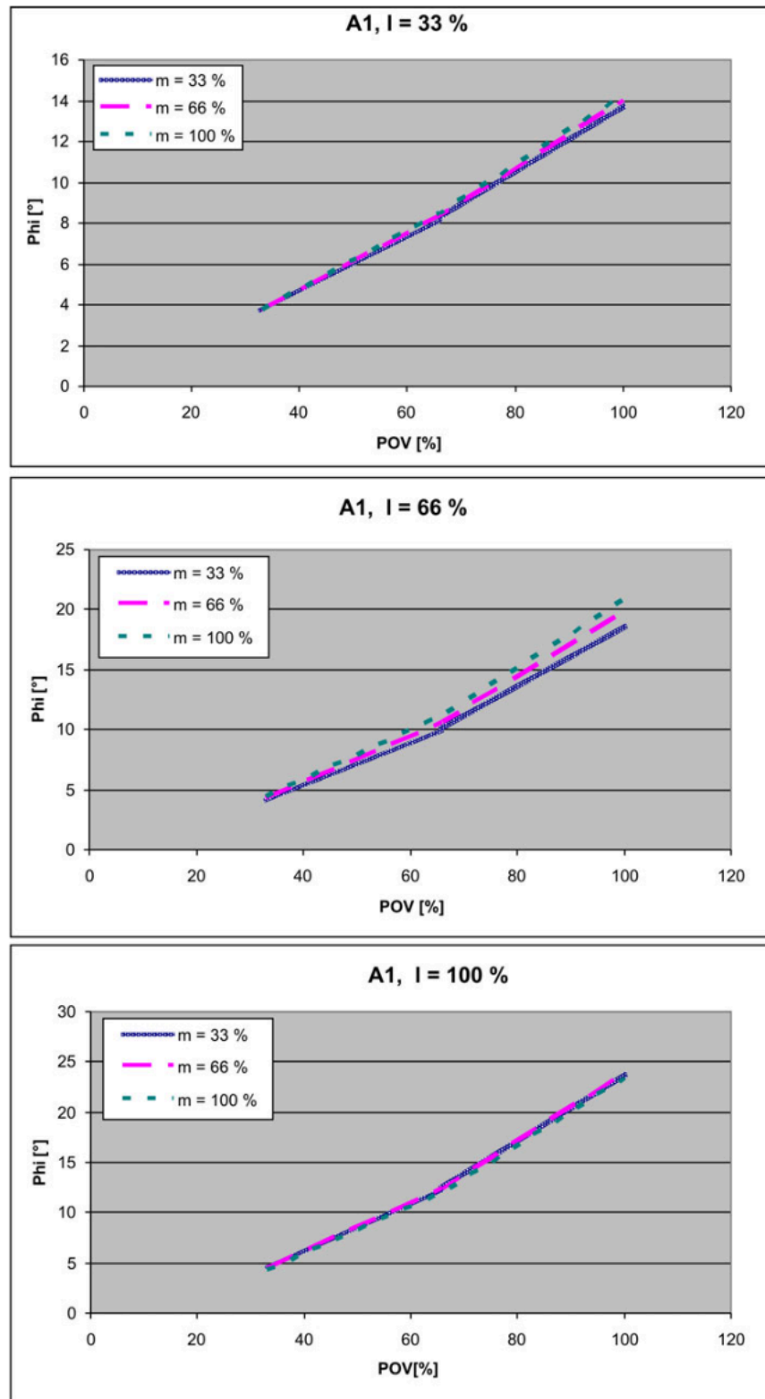
Fig. 4-11: Stopping distances for STOP 1, axis 1
