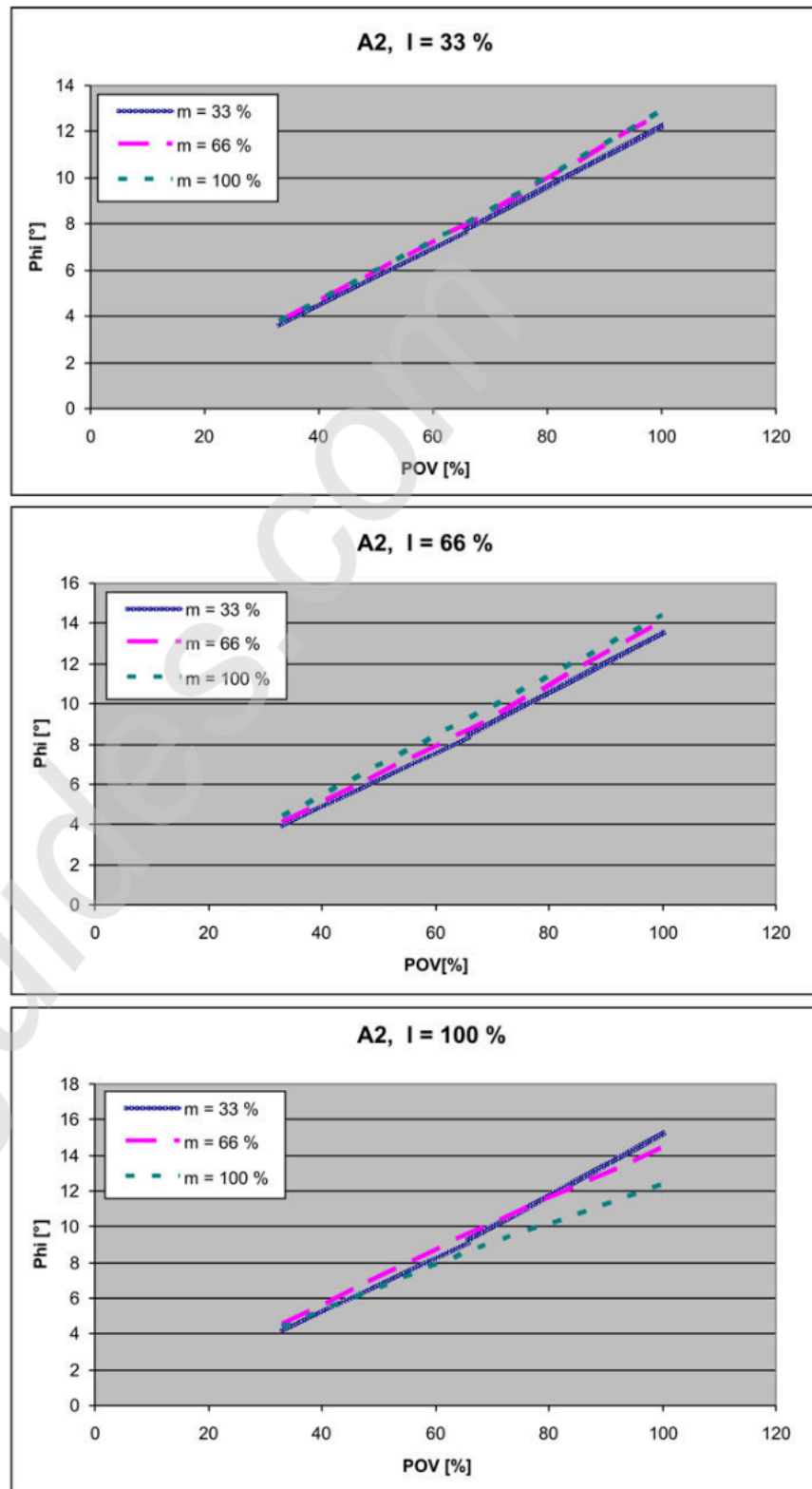
Fig. 4-21: Stopping distances for STOP 1, axis 2
