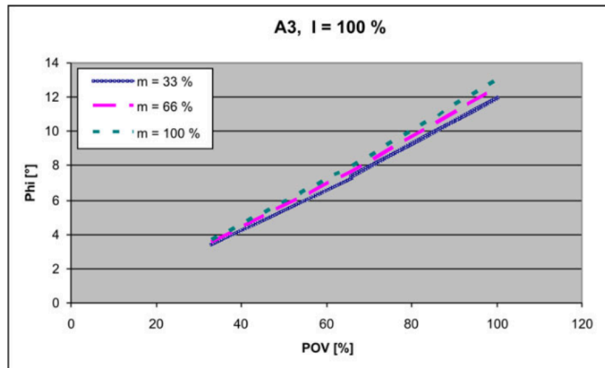
Fig. 4-19: Stopping distances for STOP 1, axis 3
