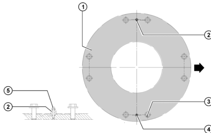
Fig. 8-7: Installing the mounting base
