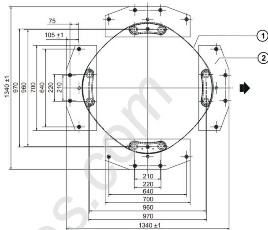
Fig. 6-5: Mounting base 200 mm, dimensioned drawing
