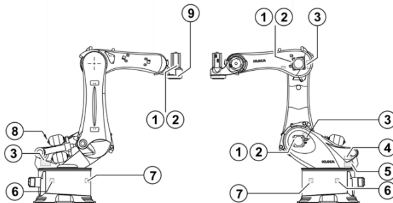
Fig. 4-9: Location of plates and labels
