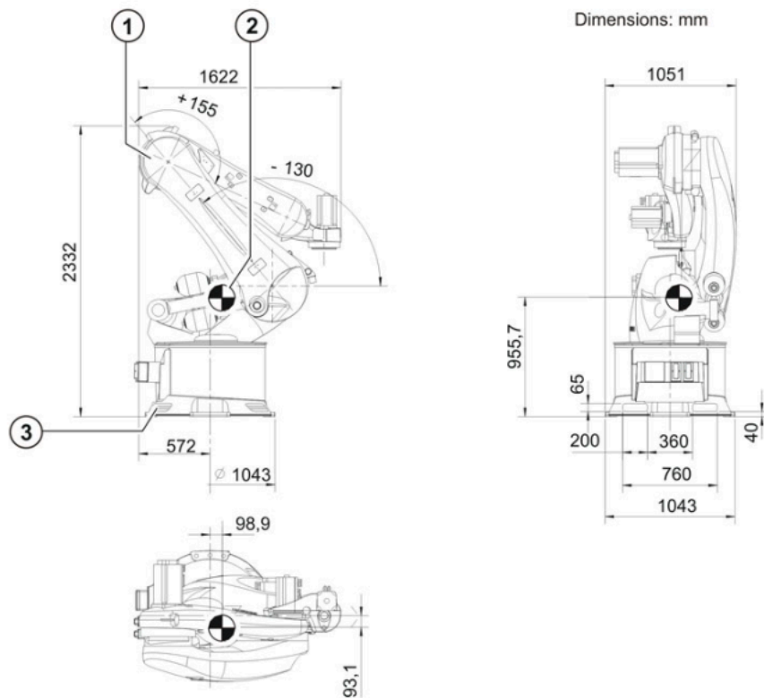
Fig. 4-8: Transport dimensions
