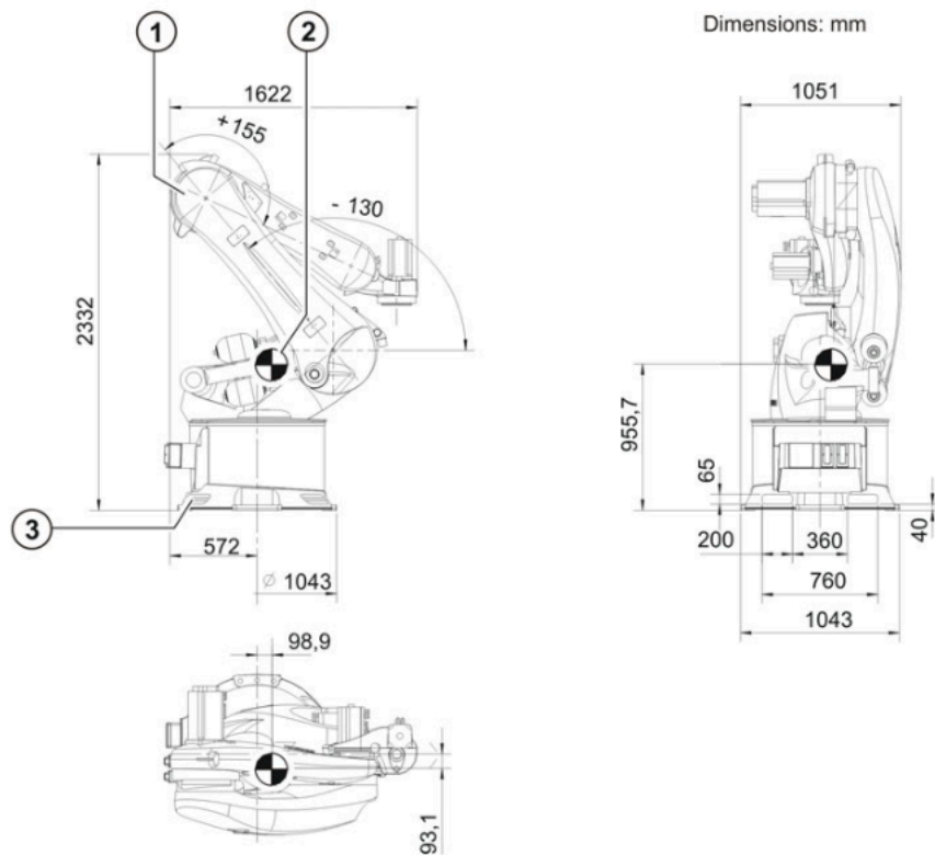
Fig. 7-2: Transport dimensions
