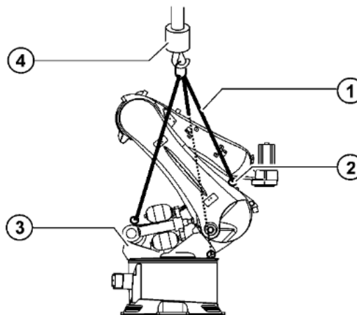
Fig. 7-4: Transportation using lifting tackle
