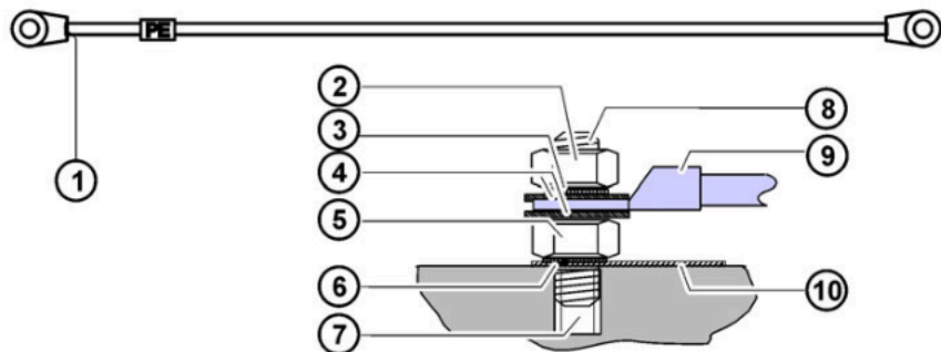
Fig. 8-16: Connecting cable, ground conductor
