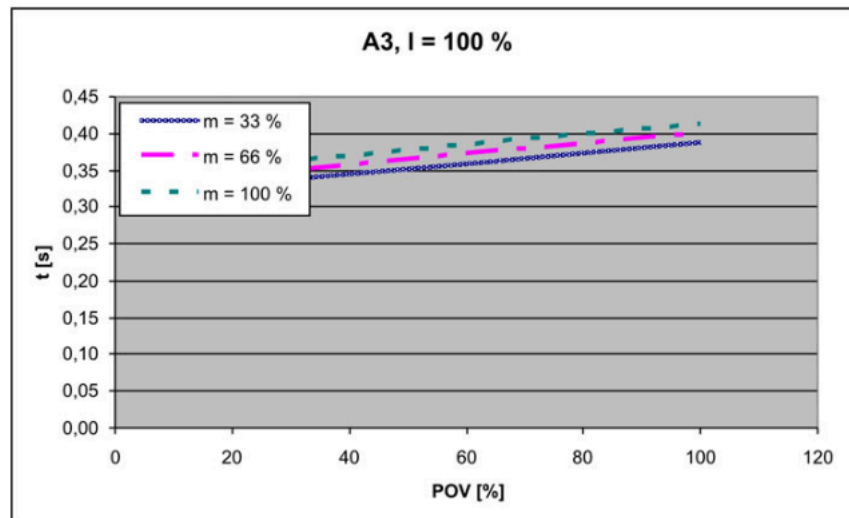
Fig. 4-20: Stopping times for STOP 1, axis 3
