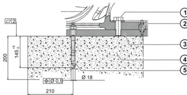
Fig. 6-6: Cross-section of foundation 200 mm
