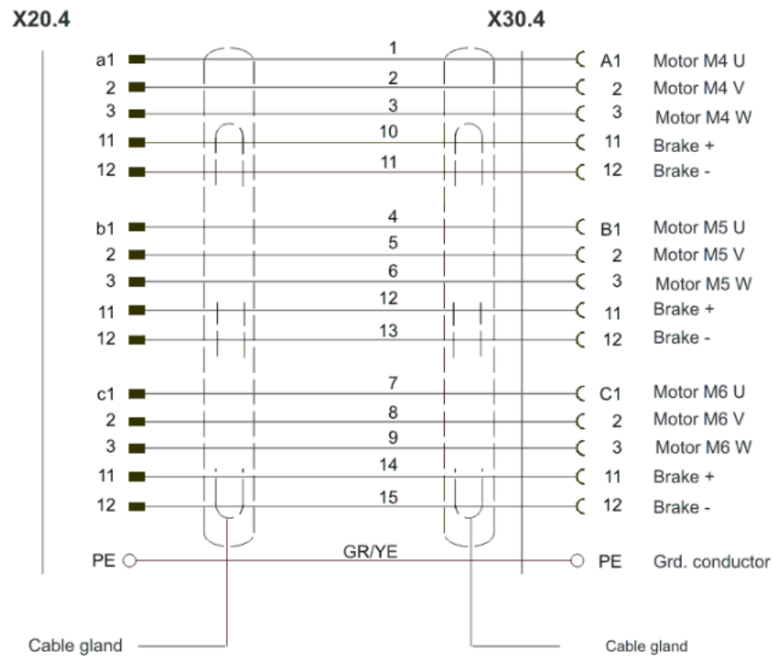
Fig. 8-13: Wiring diagram, motor cable X20.4-X30.4
