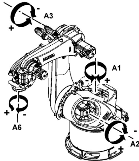
Fig. 4-1: Direction of rotation of robot axes
