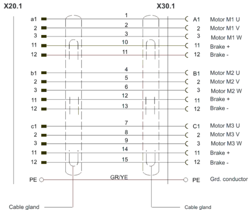
Fig. 8-11: Wiring diagram, motor cable X20.1 - X30.1
