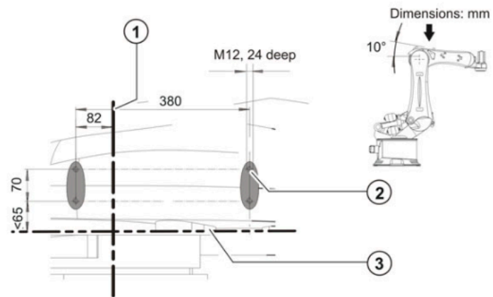
Fig. 4-6: Supplementary load on arm
