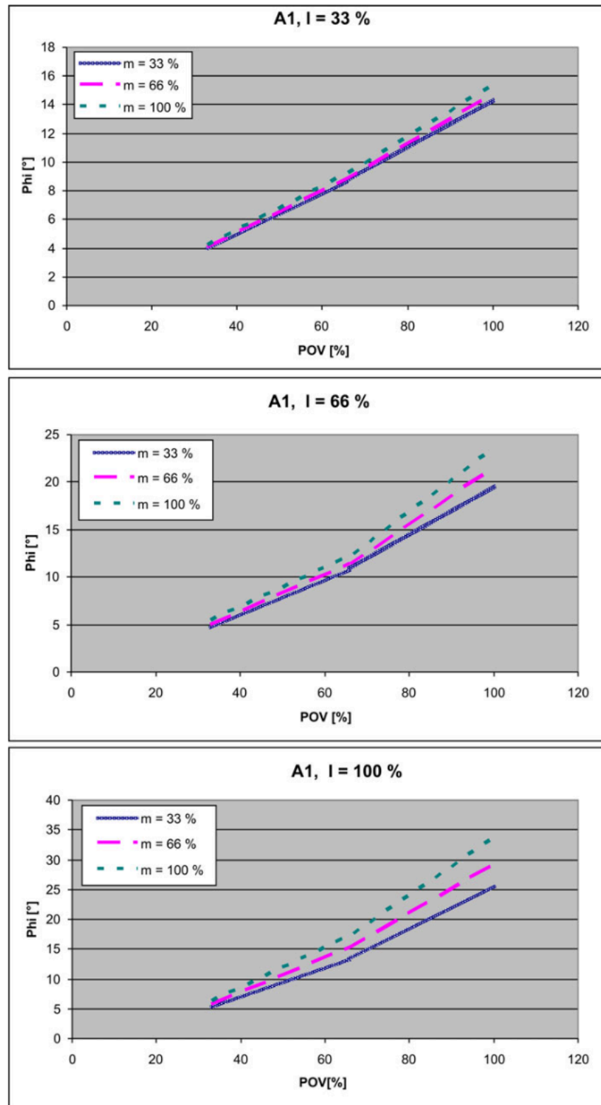
Fig. 4-17: Stopping distances for STOP 1, axis 1
