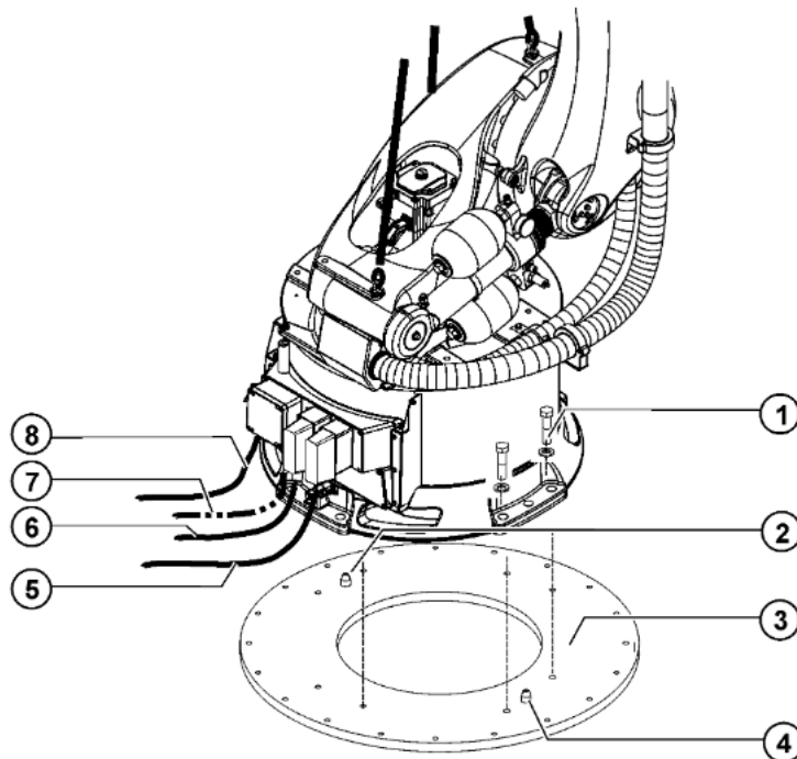
Fig. 8-8: Installing the robot
