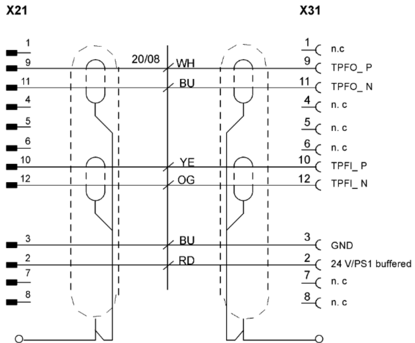
Fig. 8-15: Connecting cable, wiring diagram, data cable X21 - X31
