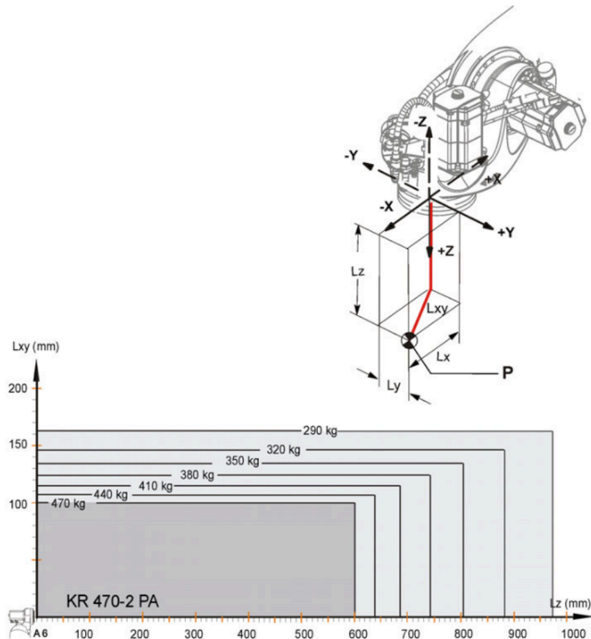
Fig. 4-4: Payload diagram for KR 470-2 PA
