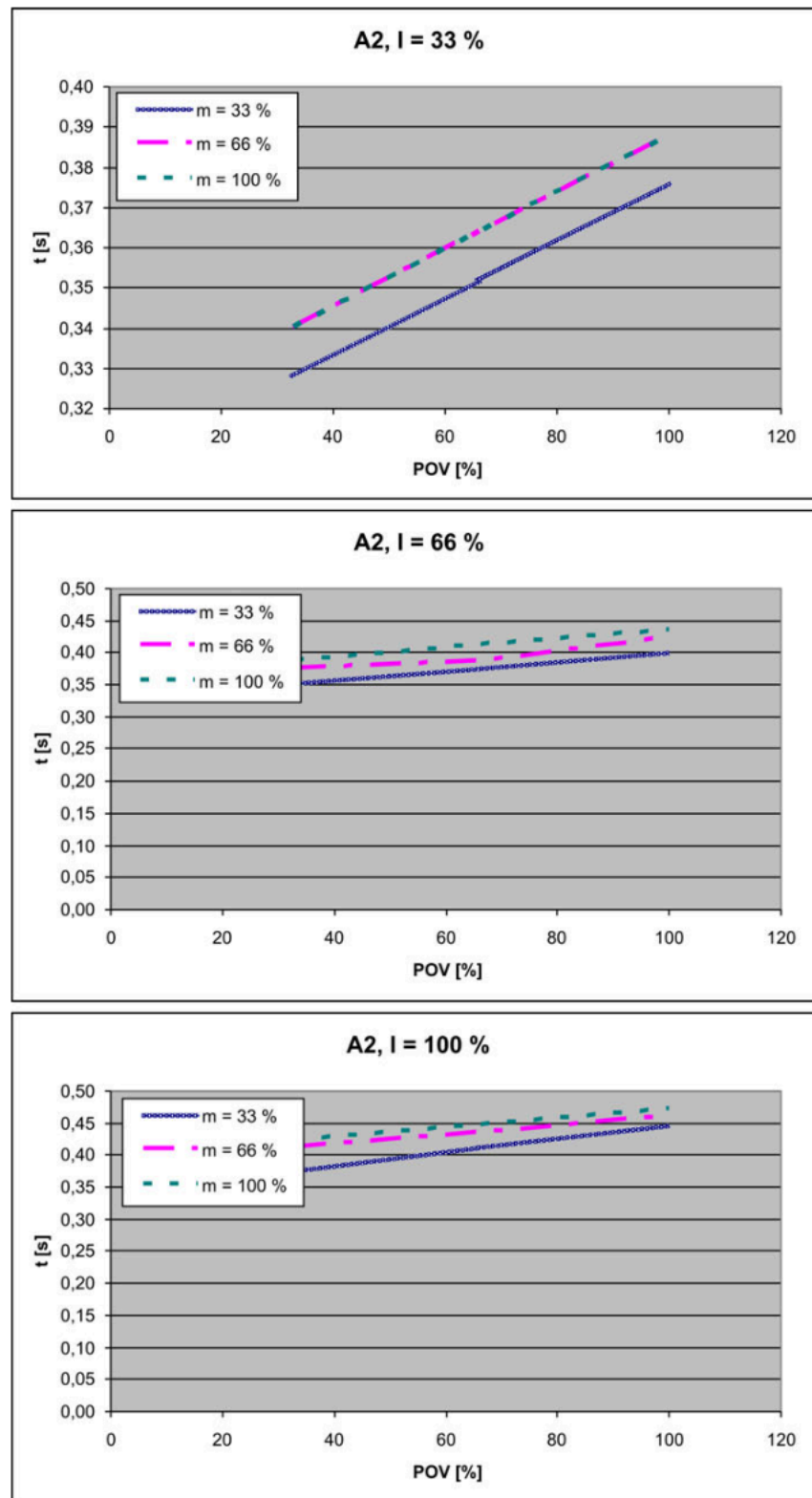
Fig. 4-22: Stopping times for STOP 1, axis 2
