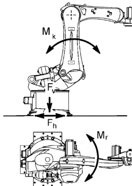
Fig. 4-7: Loads acting on the foundation
