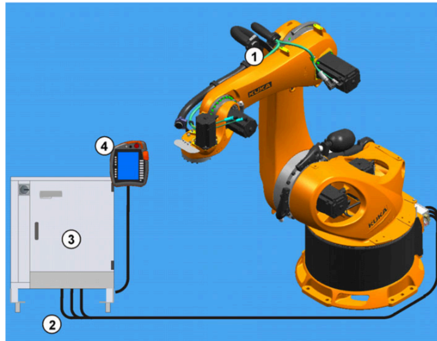
Fig. 3-1: Robot system KR 300, 470-2 PA
