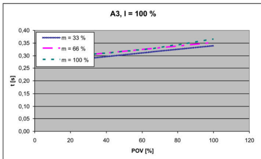
Fig. 4-16: Stopping times for STOP 1, axis 3
