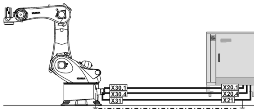
Fig. 8-9: Connecting cables, overview
