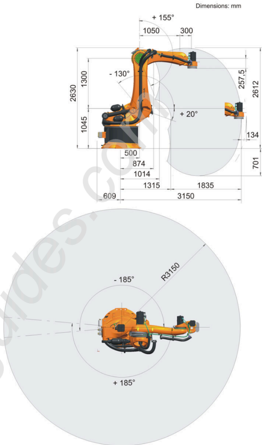
Fig. 4-2: Working envelope: KR 300 470 PA
