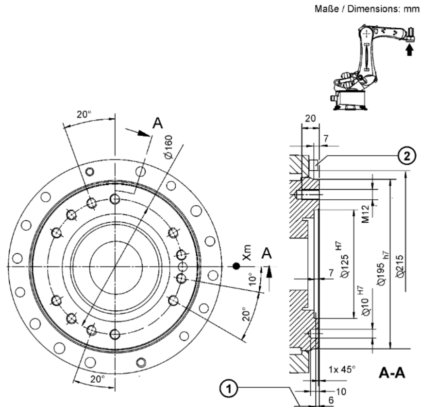
Fig. 4-5: Mounting flange
