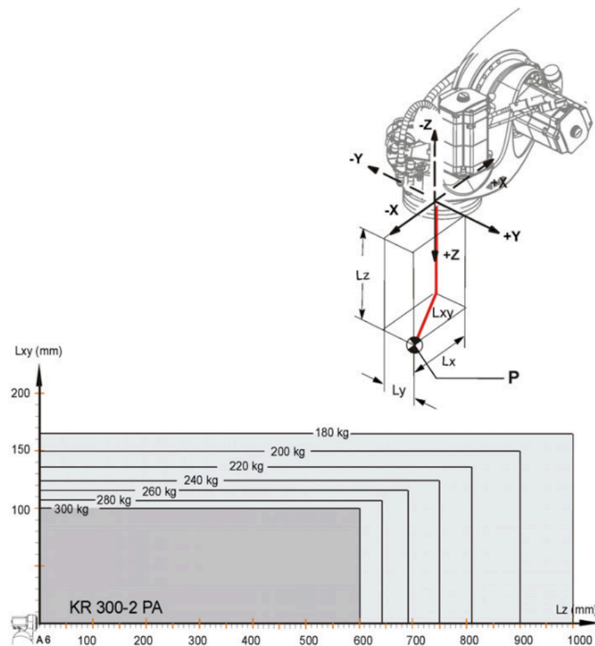
Fig. 4-3: Payload diagram for KR 300-2 PA
