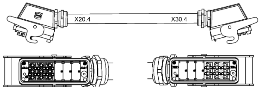
Fig. 8-12: Connecting cable, motor cable, X20.4 - X30.4
