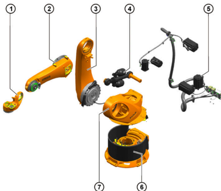
Fig. 3-2: KR 300 470-2 PA: main assemblies
