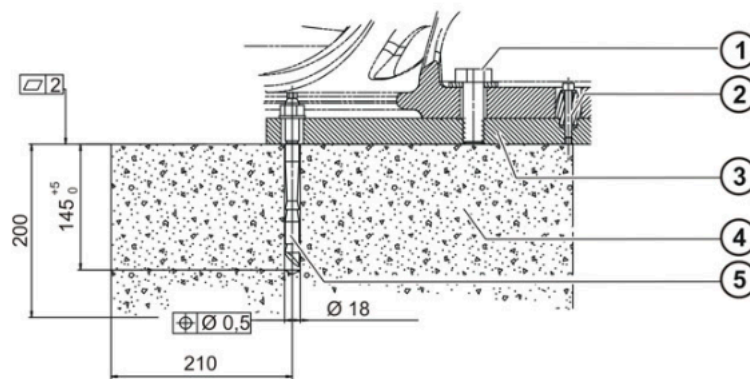
Fig. 8-6: Cross-section of foundation 200 mm
