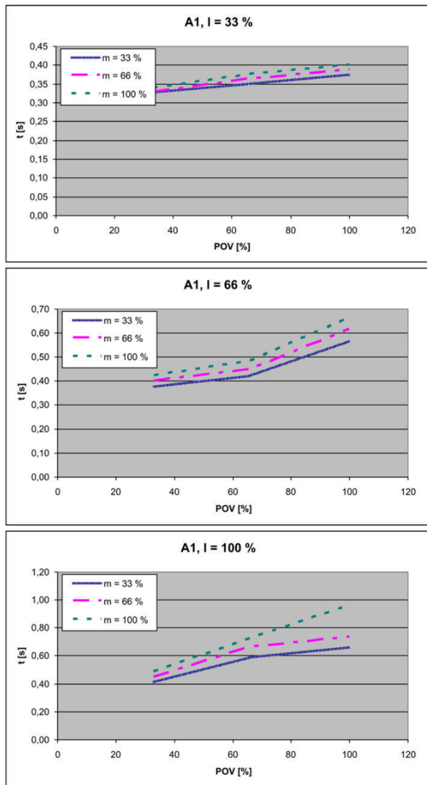
Fig. 4-18: Stopping times for STOP 1, axis 1
