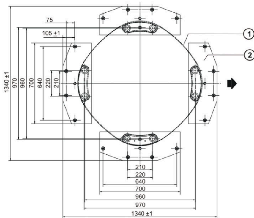
Fig. 8-5: Mounting base 200 mm, dimensioned drawing
